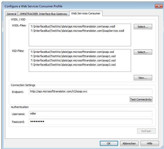
You can integrate web services by simple configuration in the Web Services Consumer.
