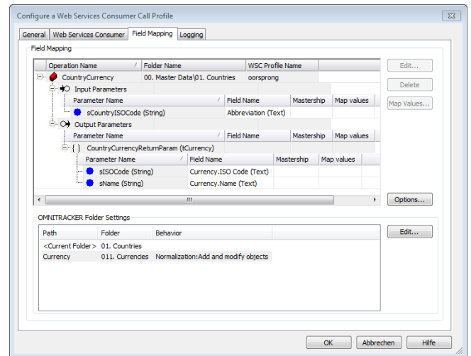
Operation calls can be configured in profiles.
